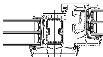
V7 = A046/76302(V319) - A036/76200(V315) - 76509
