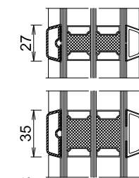
L5 = 27 mm (A244T, 92001), 35 mm (A246T, 92003) VS = 27 mm (A243T, 92000), 35 mm (A245T, 92002)
