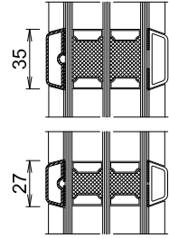
LS = 27 mm (A244T, 92001), 35 mm (A246T, 920)
