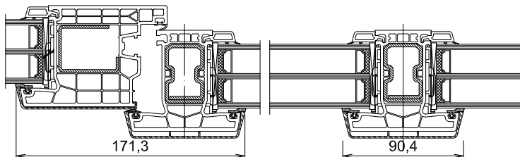
V3 = A038/76200(V315) - A046/76302(V319) - 76509
