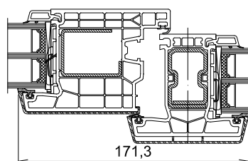
V3 = A038/76204(V326) - A046/76302(V319) - 76509
