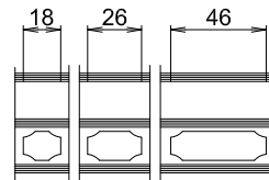
LS, VS = ilagt sprosse 18 mm, 26 mm, 46 mm
