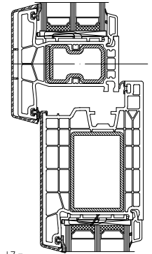
L7 = A046/76302(V319) - A040/76206(V260) - 76509
