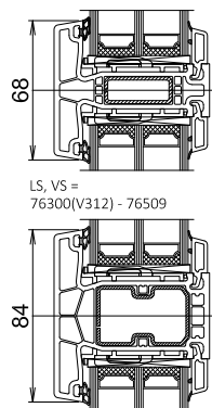
LS, VS = 76302(V343) - 76509
